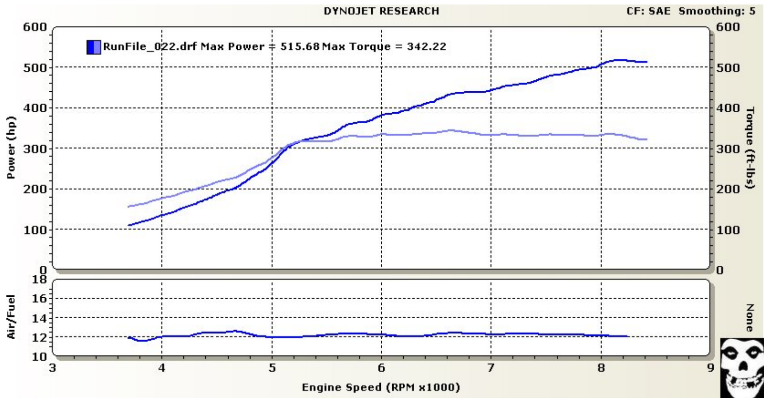
Figure 6. GT3040 @ 19 psi on race gas blend fuel.
