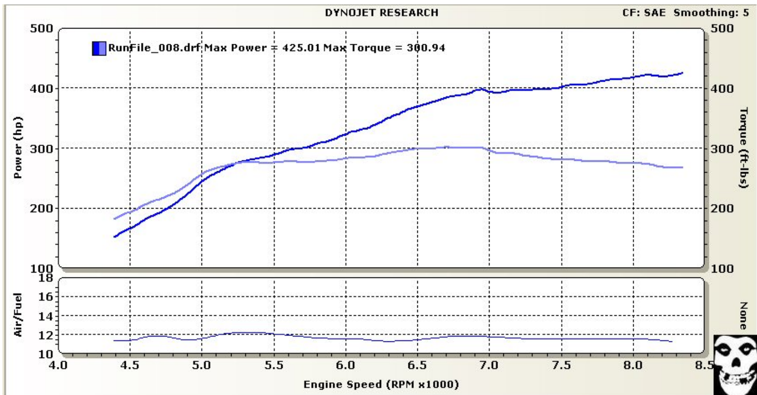
Figure 5. GT3040 @ 15 psi on pump gas.
